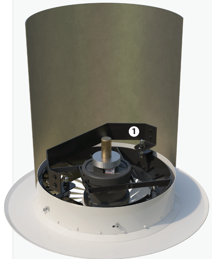
Figure 6 - Installation of an HSC-AD (shown with thermal element) into a round duct with mounting bracket ① using 2pcs M6 bolts accessible through the diffuser face. Suitable for sizes DN250-DN500 with electric, thermal or manual adjustment.
