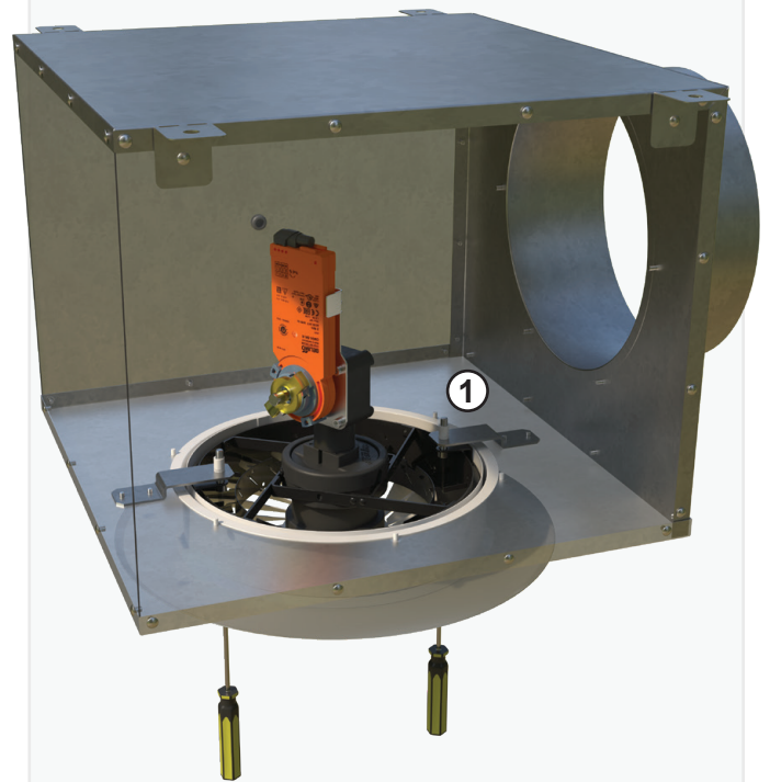
Figure 4 - Installation of an HSC-AD (shown with electric adjustment) into a plenum box using 2pcs M6 bolts ① accessible through the diffuser face. Suitable for sizes DN250-DN500 with electric, thermal or manual adjustment.
